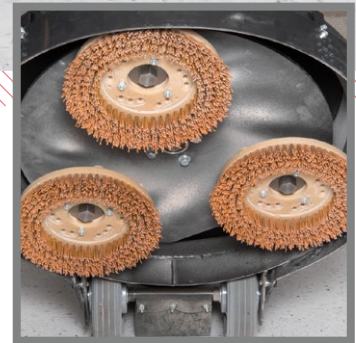
3 counter rotating brushes allow for one pass stripping
